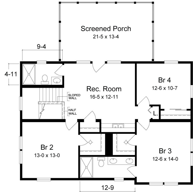
SECOND FLOOR
